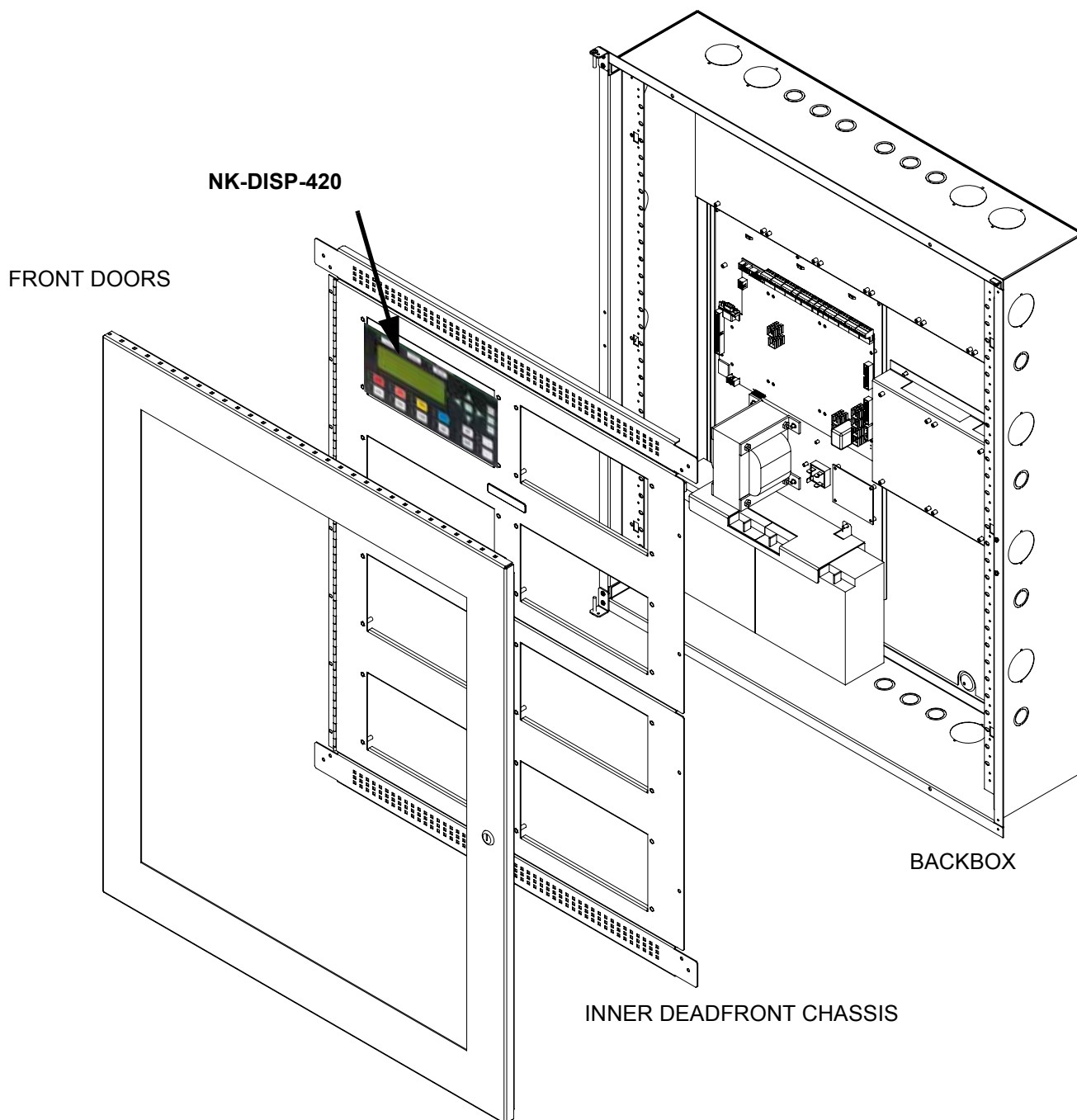
Figure 1: NK-DISP-420 Mounted in the NK-7000LBB Enclosure
